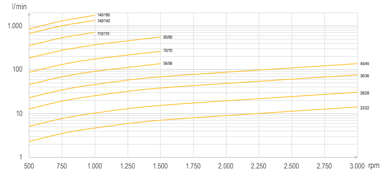
refinex® refiftherm® 22-140 flow rate @ 0 bar ΔP
